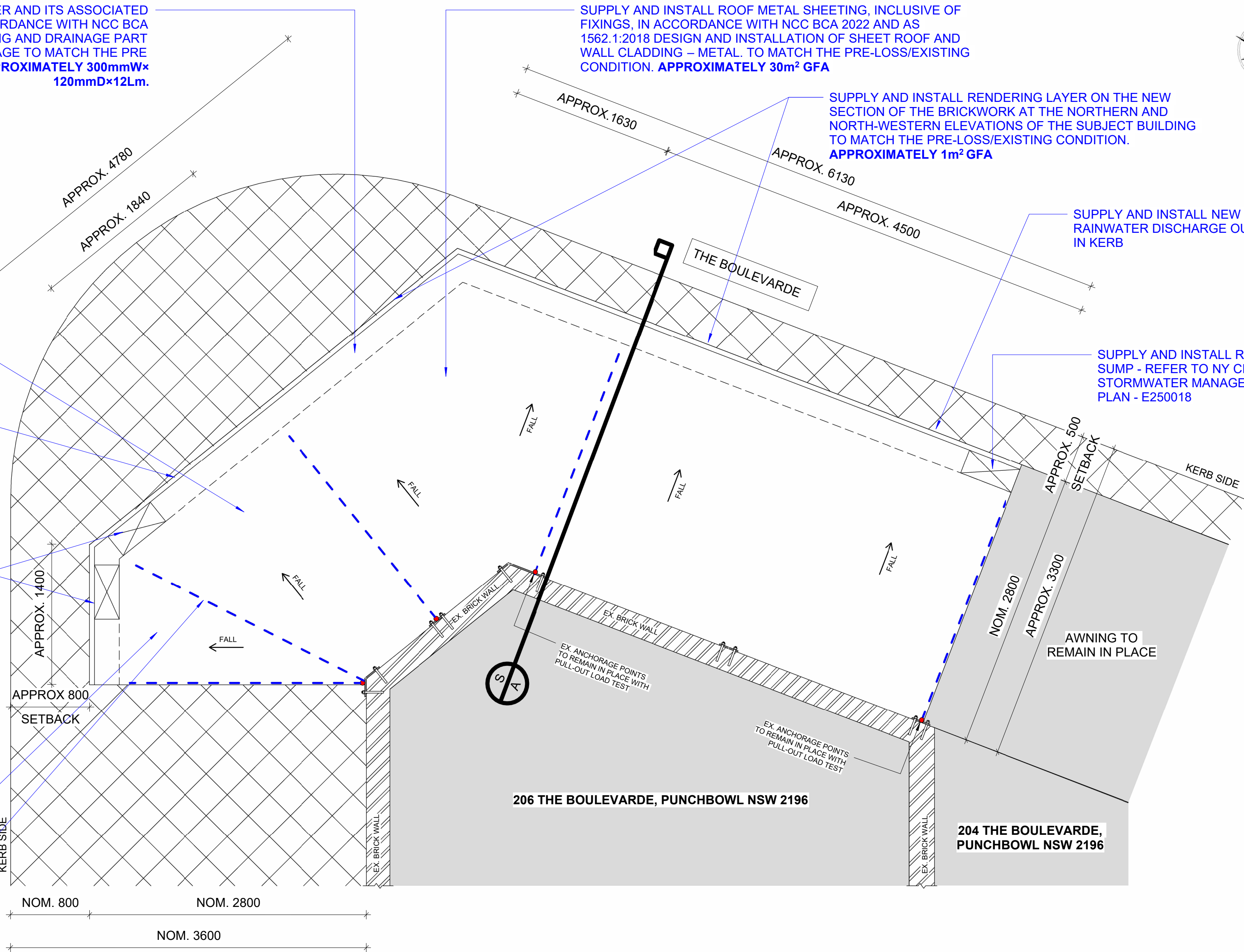
1 PROPOSED PLAN 1 : 30
